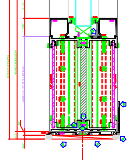
214 SIDE LITE BASE 25/25/25/25
