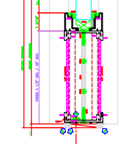
214 SIDE LITE BASE 25/25/25/25
